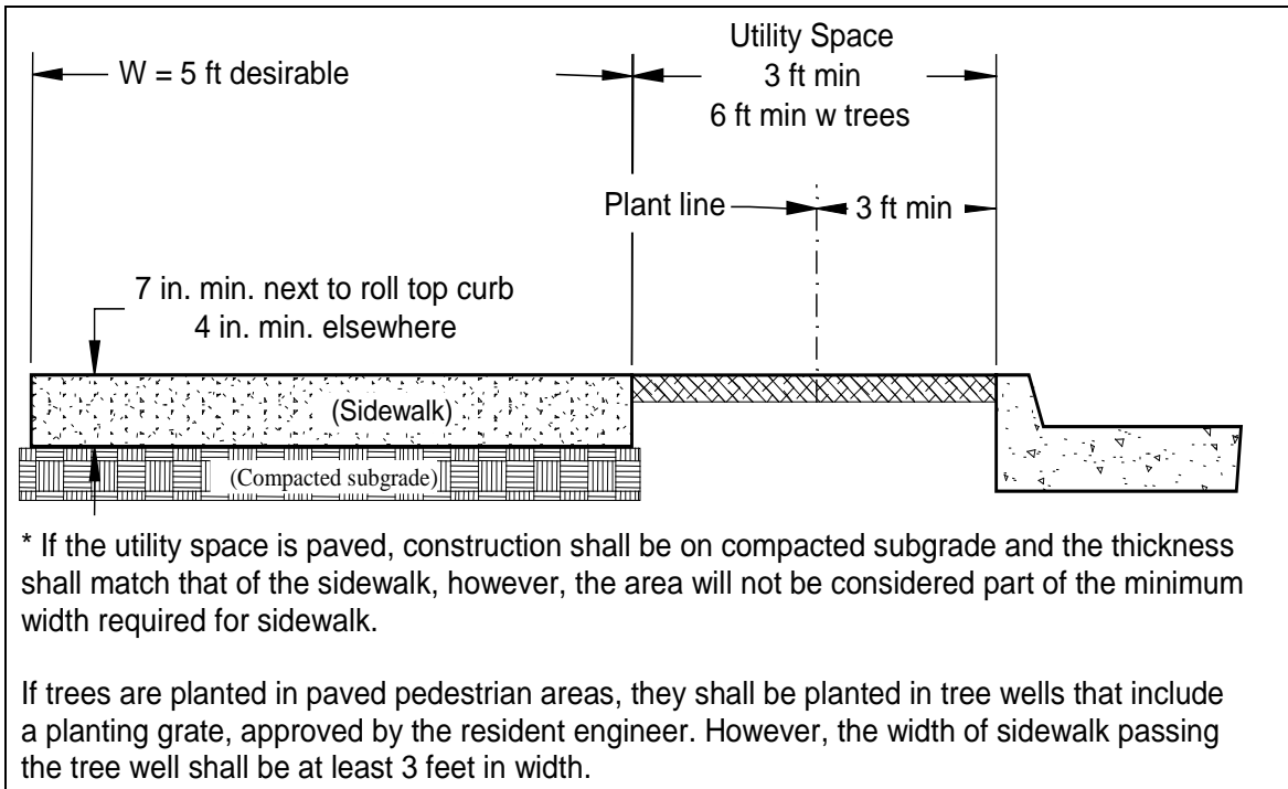
FIGURE 6 –DETAIL BACK OF CURBS
