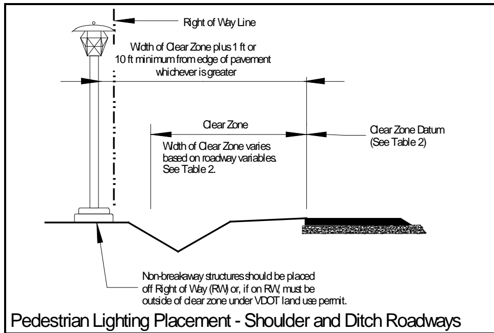
FIGURE 14 – LIGHTING ALONG SHOULDER AND DITCH SECTIONS
