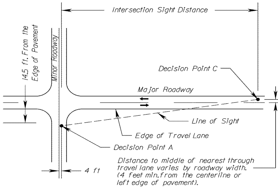
Right Sight Distance Triangle
