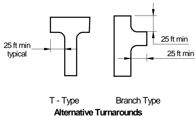
FIGURE 4 – CUL-DE-SAC DETAILS*
