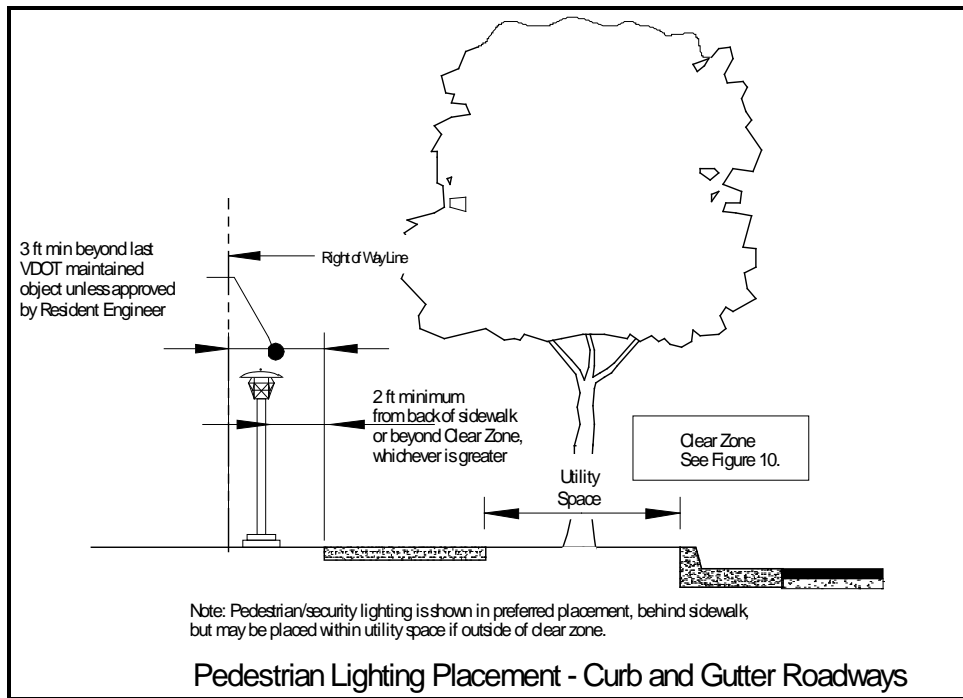
FIGURE 13 – LIGHTING ALONG CURB AND GUTTER SECTIONS
