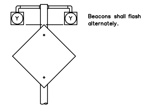
BEACON ALIGNMENT DETAIL
