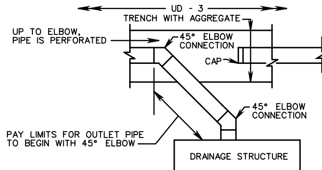
OUTLET PIPE
